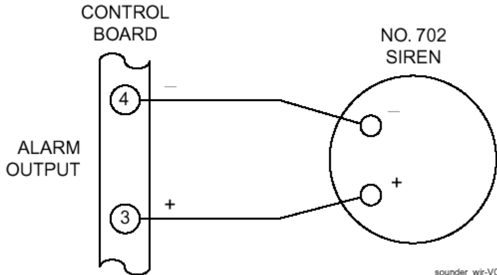
Figure 2-6. Typical Sounder Wiring
